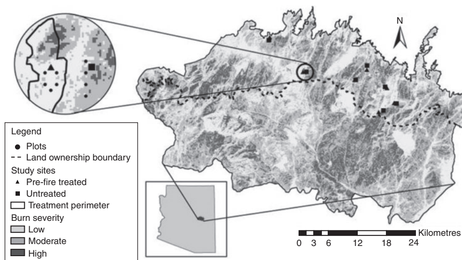
Fig. 1. Map of the Rodeo–Chediski Fire in east-central Arizona. Map taken from Shive et al. (2013b).
