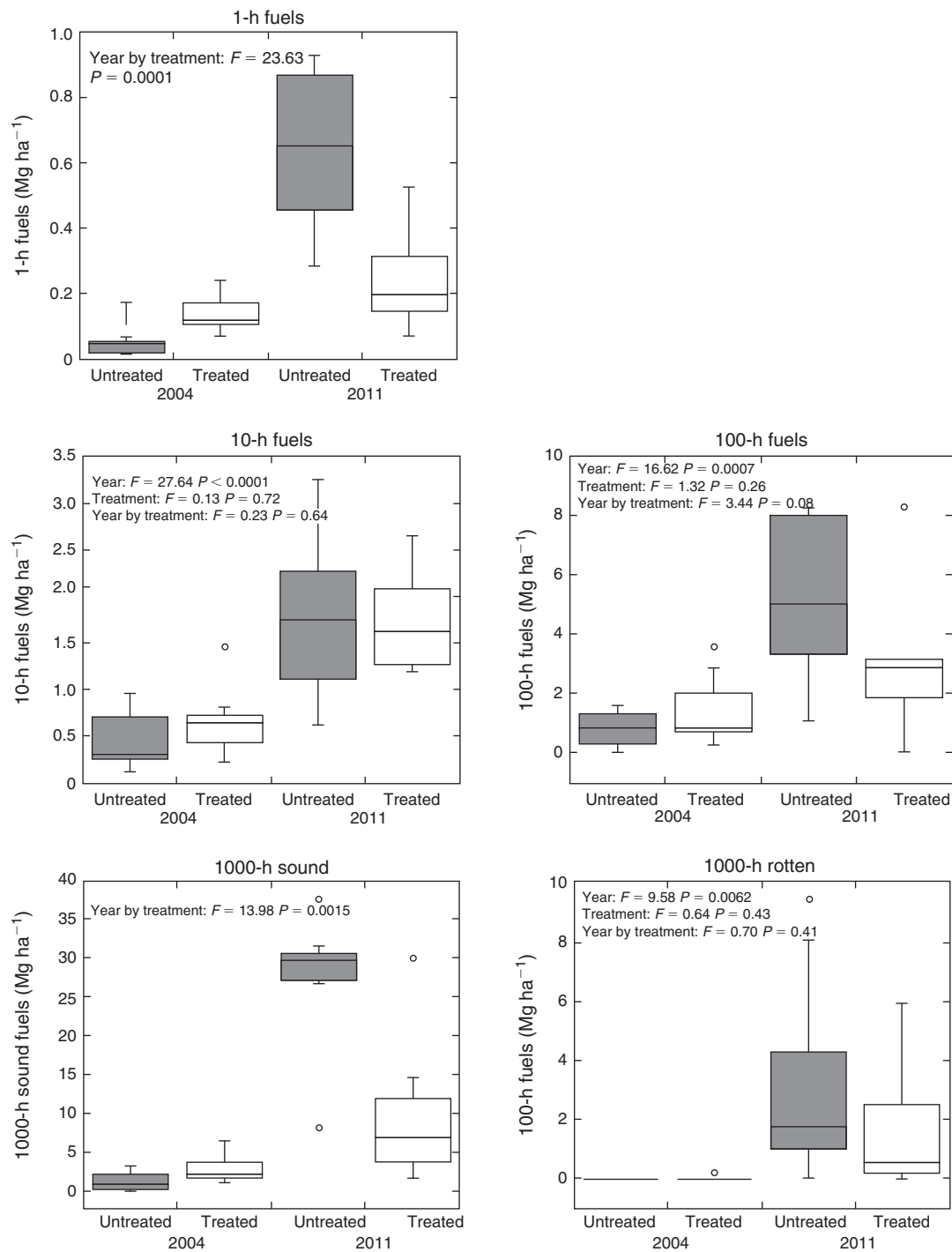
Fig. 2. Surface fuel characteristics: grey box plots indicate untreated sites; clear box plots indicate treated sites. Clear circles identify outliers and T-bars indicate the 75th percentile. The 2004 data are shown on the left of each graph and 2011 data are on the right. F - and P -values are from the repeated-measures ANOVA, showing the year, treatment and year-by-treatment interaction values.
