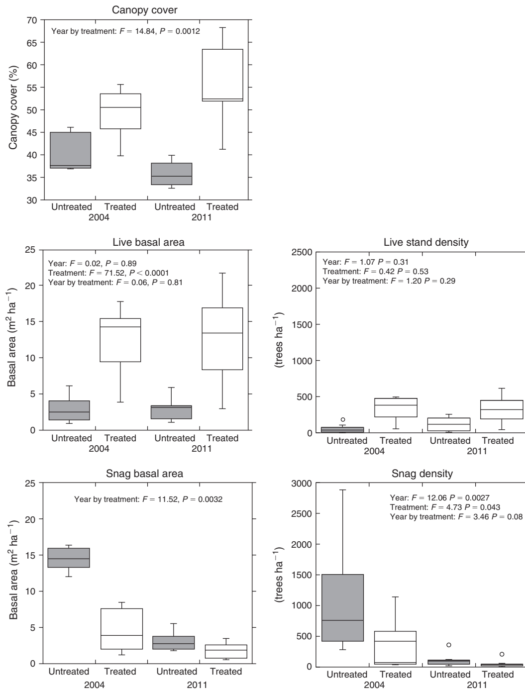
Fig. 3. Canopy fuel characteristics: canopy cover, live basal area and tree density, snag basal area and tree density: grey box plots indicate untreated sites; treated sites are represented by clear box plots. Clear circles identify outliers and T-bars indicate the 75th percentile. The mid-line indicates the mean. The 2004 data are shown on the left of each graph and 2011 are on the right. F - and P -values are from the repeated-measures ANOVA, for year and treatment main effects and year-by-treatment interaction.
