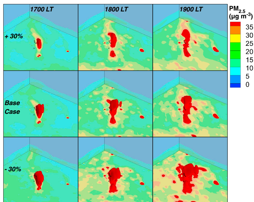
Figure 8. Modeled pollution plumes on 28 February 2007 (LT) shown as three-dimensional isosurfaces bound by PM 2.5 concentration equal to 35 \mu\text{g m}^{-3} for base case and simulations carried out with \pm 30\% perturbations to wind speed. Ground-level PM 2.5 concentrations ( \mu\text{g m}^{-3} ) are also shown. Air quality monitoring sites are indicated by black markers.
