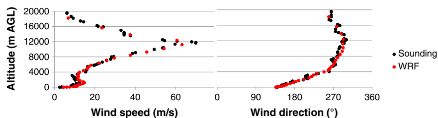
Figure 13. Wind speed and direction predicted by WRF (red) upper air observations (black) from the rawinsonde launched from Peachtree City, GA at 1900 LT on 28 February 2007.
