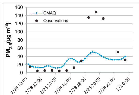
Figure 1. Observed 1 h average and CMAQ-predicted 15 min PM 2.5 concentrations at the Confederate Ave. monitoring site on 28 February 2007 (LT).
