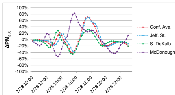
Figure 4. Change in CMAQ-predicted PM 2.5 concentrations on 28 February 2007 (LT) relative to base case simulation at the Confederate Ave., Jefferson St., South DeKalb, and McDonough monitoring sites after applying a -5^\circ perturbation to wind direction.
