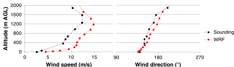
Figure 14. WRF-predicted wind speed and direction and observations from the rawinsonde launched from Peachtree City, GA at 1900 LT on 28 February 2007 for lower 2000 m of the atmosphere.
