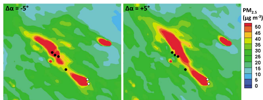
Figure 5. CMAQ-predicted PM 2.5 concentrations ( \mu\text{g m}^{-3} ) over northern Georgia at 1900 LT on 28 February 2007 using -5^\circ and +5^\circ perturbations to wind direction. Black shaded circles indicate monitoring station locations. The Oconee and Piedmont fire sites are denoted by white shaded markers.
