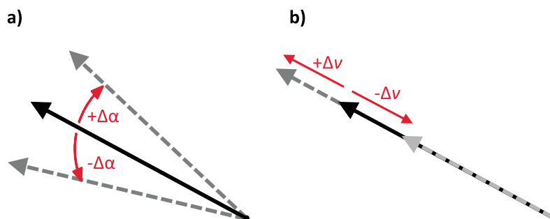
Figure 2. Representation of perturbations applied to (a) wind direction and (b) wind speed in brute-force sensitivity analyses.
