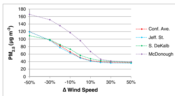
Figure 7. Maximum CMAQ-predicted PM 2.5 concentrations at the Confederate Ave., Jefferson St., South DeKalb, and McDonough monitoring sites with wind speed perturbations ranging from -50\% to +50\% .
