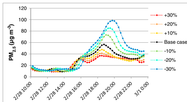
Figure 6. CMAQ-predicted PM 2.5 concentrations on 28 February 2007 (LT) at the South DeKalb monitoring site with wind speed perturbations. Base case simulation results are also included.
