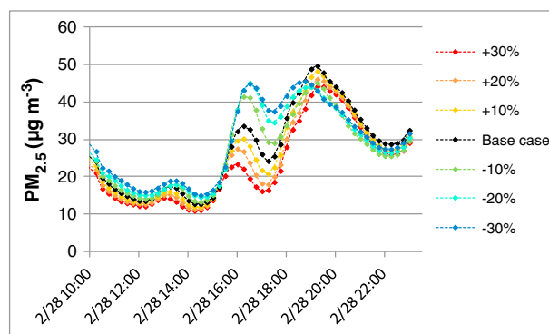
Figure 10. CMAQ-predicted PM 2.5 concentrations on 28 February 2007 (LT) at the Jefferson St. monitoring site under perturbed PBL heights. Base case simulation results are also included.
