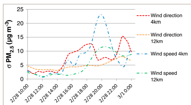
Figure 9. Standard deviation of PM 2.5 concentration from CMAQ predictions on 28 February 2007 (LT) at Confederate Ave. for all simulations within the perturbation range applied to wind direction ( \pm 5^\circ , \pm 15^\circ , \pm 30^\circ , and base case) and wind speed ( \pm 10\% , \pm 20\% , and \pm 30\% , and base case) under 4 km and 12 km horizontal grid resolutions.
