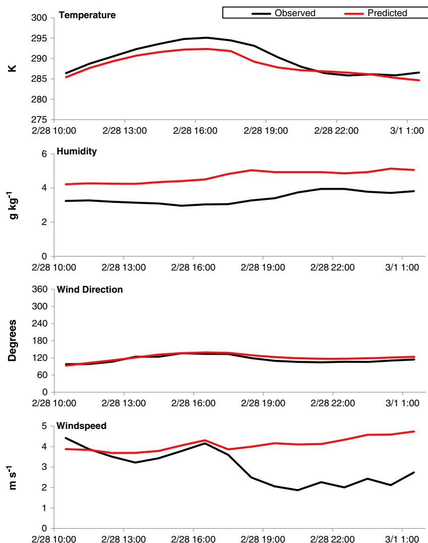
Figure 12. Mean observed and WRF-predicted ground-level temperature, humidity, wind direction, and wind speed over northern Georgia for 15 h starting at 1000 LT on 28 February 2007.
