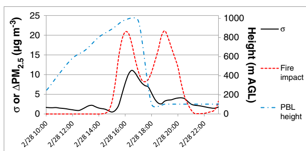
Figure 11. Standard deviation ( \sigma ) of CMAQ-predicted PM 2.5 concentrations on 28 February 2007 (LT) for all simulations carried out under different PBL heights ( \pm 10\% , \pm 20\% , and \pm 30\% , and base case) and base case PBL height prediction at Confederate Ave. (right vertical axis). The estimated fire-related contribution to PM 2.5 concentration ( \Delta PM_{2.5} ) is also included.
