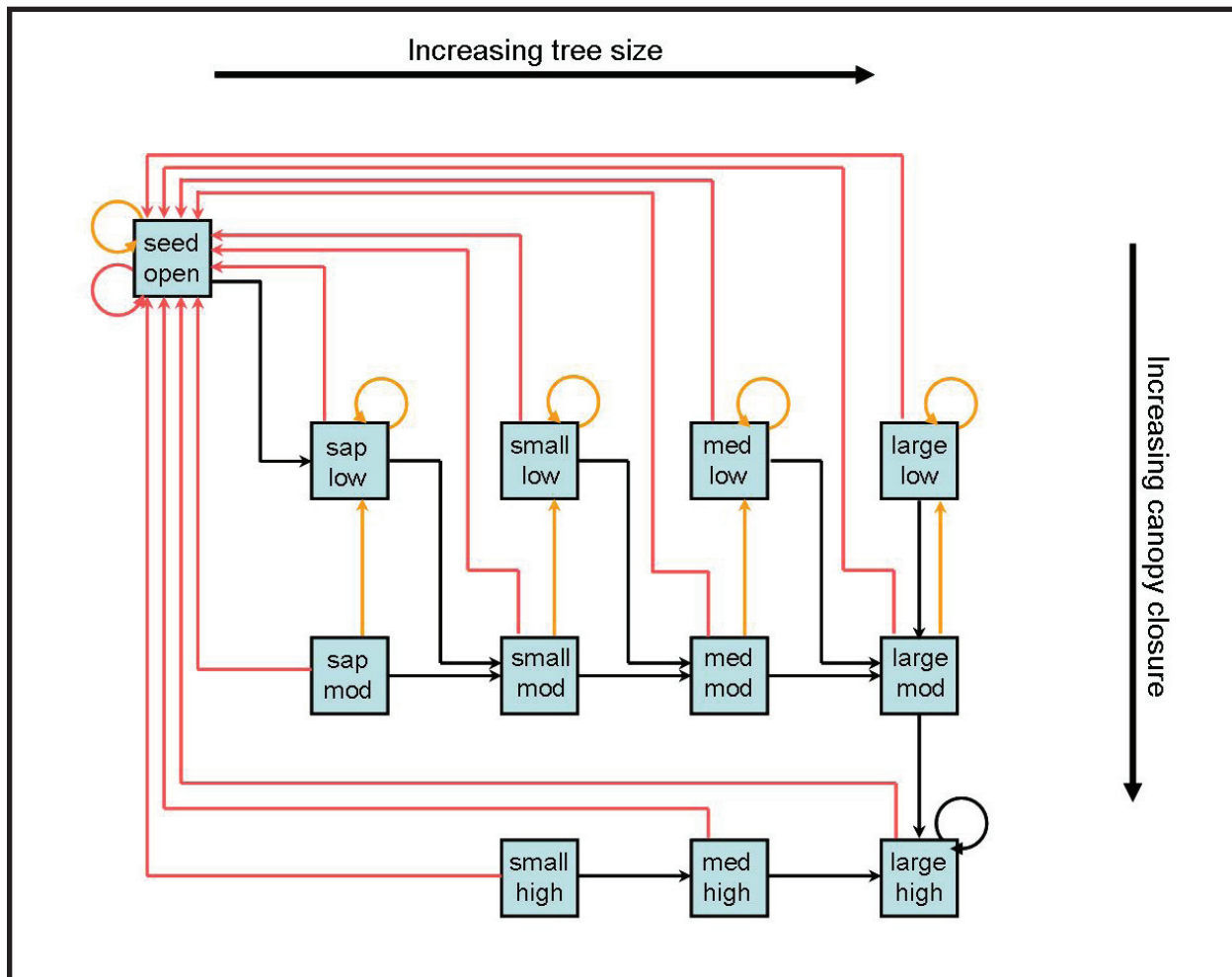
Figure 2. The successional pathway diagram for PVG 7 (warm-dry sub-alpine fir) showing possible transitions due to succession and fire among 12 successional states. Deterministic successional transitions are shown as black lines; transitions resulting from stochastic non-lethal and stand-replacing fires are shown in orange and red, respectively. Each state is defined by one of five tree size classes (see Tables 1 and 3) and one of four canopy closure classes: open (<10 %), low (10 % to 39 %), moderate (40 % to 69 %), and high (>69 %).
