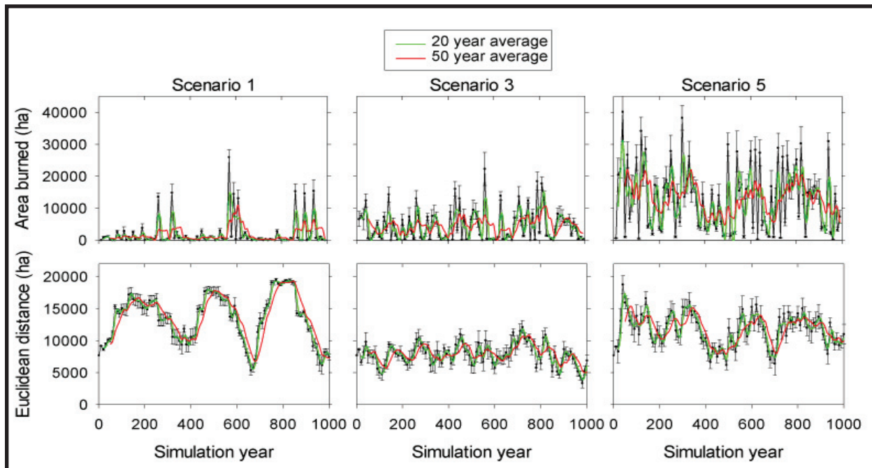
Figure 4. Area burned and Euclidean Distance for Scenarios 1, 3 and 5 in 10-year intervals. Year 0 represents current conditions. Average of 10 replicate simulations shown, error bars reflect standard deviation among 10 replicates. Twenty-year and 50-year running averages displayed in green and red, respectively.
