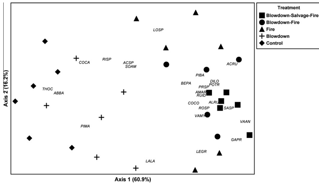
Fig. 5. Non-metric multidimensional scaling (NMS) ordination of woody species composition across disturbance treatments. Species locations in ordination space are based on weighted averaging and codes are defined in Appendix A (available online). See Appendix B (available online) for species correlations with NMS axes 1 and 2.
